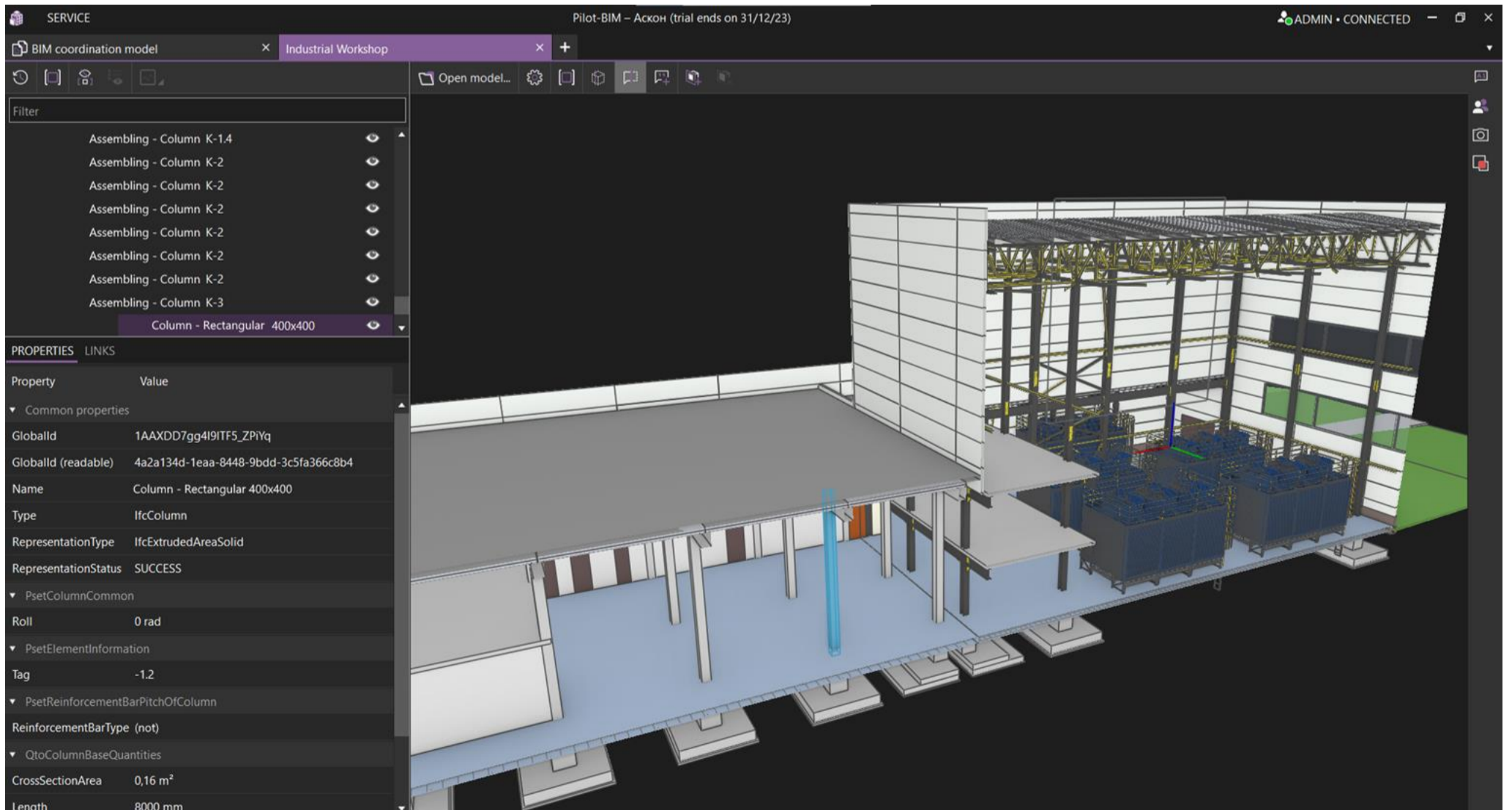
BIM-Object properties in consolidated model window
